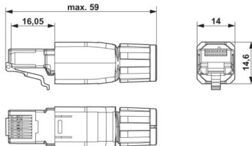
RJ45 plug connector, IP20
